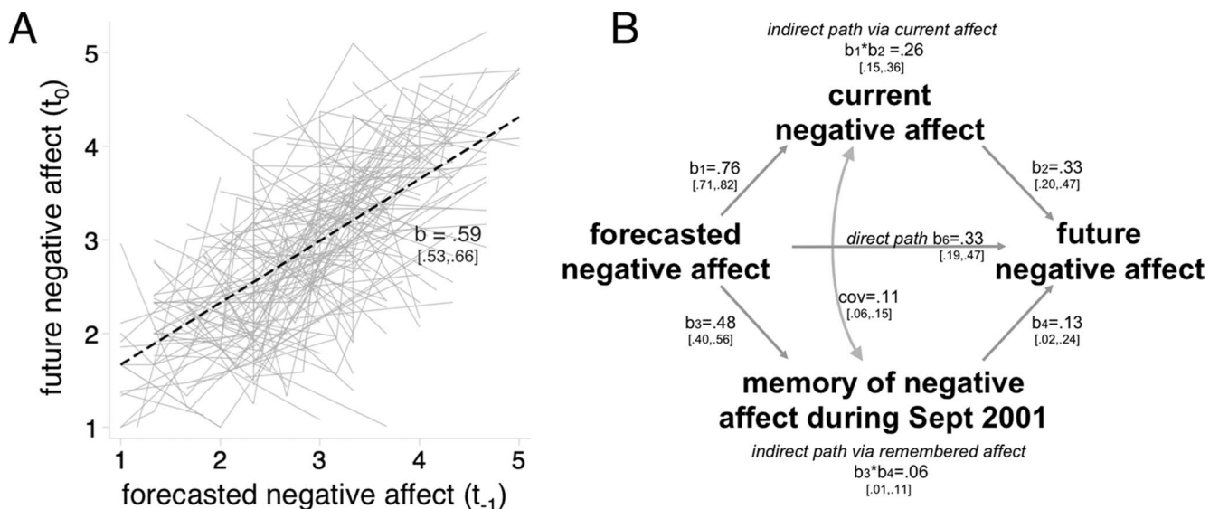
Figure 4. (A) Total predictive relationship between forecasted negative affect (at a particular time point) and experienced negative affect (at the following time point, for which the prediction was made), shown for the group as a whole (dotted black line), and in terms of raw individual curves (light gray lines). (B) Multilevel path model identifying mediators of the relationship between forecasted future negative affect and actual future negative affect. Results indicate that current feelings and memories of feelings from September 2001 independently mediate the relationship between forecasted and experienced negative affect. Unstandardized betas with 95% confidence interval.
