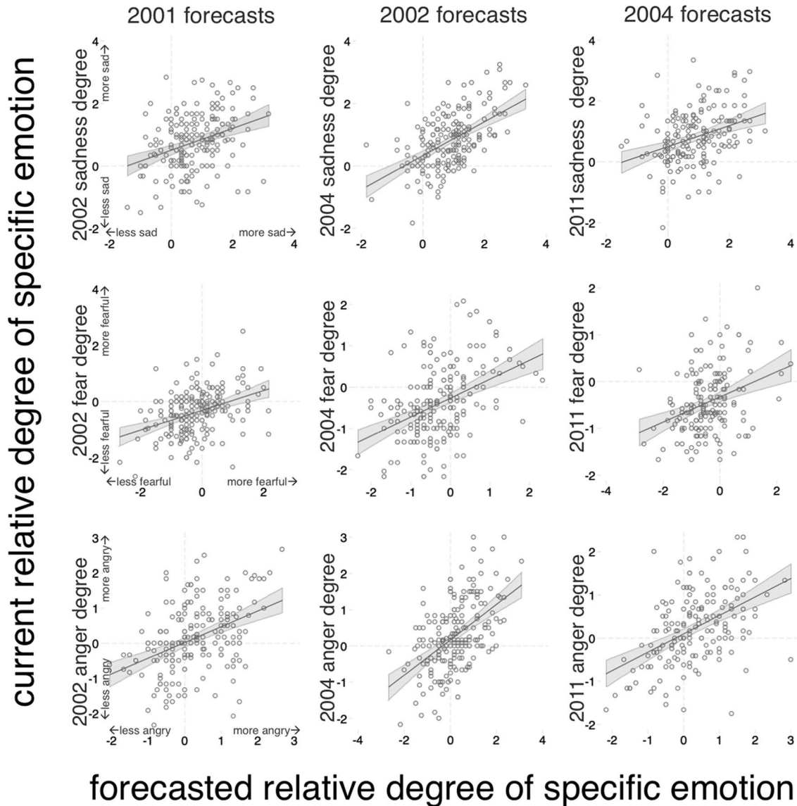
Figure 3. Relationships between the relative degree of specific types of emotion reported in response to the attacks in 2002, 2004, and 2011 (i.e., reports of particular categories centered on the mean of all reported negative emotion, on the y axes) and forecasts of relative degree made 1, 2, and 7 years earlier (i.e., forecasts mean-centered in the same manner, on the x axes). Forecasts show a high degree of relative accuracy—people who predict that they will feel predominantly sad, angry, or fearful tend to later end up doing so.
